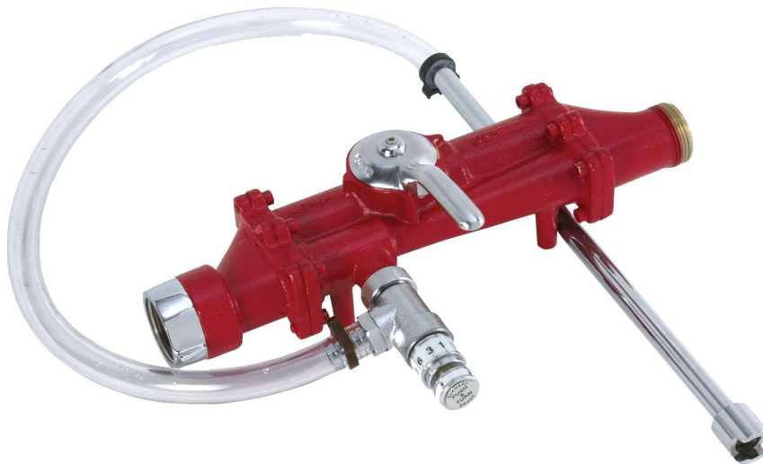
Figure 6.3: Bypass Eductor
